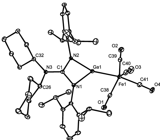
Figure 1. Molecular structure of 3 (ORTEP, thermal ellipsoids shown at 25% probability level). Hydrogen atoms omitted for clarity. Selected bond lengths [Å] and angles [°]: Ga(1)–N(1) 1.9614(18), Ga(1)–N(2) 1.9710(18), Ga(1)–Fe(1) 2.271(1), N(1)–C(1) 1.359(3), N(2)–C(1) 1.370(3), N(3)–C(1) 1.348(3); N(1)–Ga(1)–N(2) 67.94(7), C(41)–Fe(1)–Ga(1) 169.84(8), N(3)–C(1)–N(1) 126.36(18), N(3)–C(1)–N(2) 126.39(18), N(1)–C(1)–N(2) 107.24(17).
