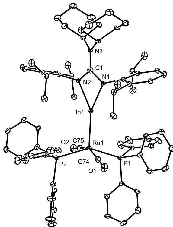
Figure 3. Molecular structure of 6 (ORTEP, thermal ellipsoids shown at 25% probability level). Isopropyl groups and hydrogen atoms omitted for clarity. Selected bond lengths [Å] and angles [°]: \text{In}(1)-\text{N}(1) 2.243(5), \text{In}(1)-\text{N}(2) 2.285(5), \text{In}(1)-\text{Ru}(1) 2.5549(9), \text{Ru}(1)-\text{C}(75) 1.906(9), \text{Ru}(1)-\text{C}(74) 1.920(8), \text{Ru}(1)-\text{P}(2) 2.337(2), \text{Ru}(1)-\text{P}(1) 2.338(2), \text{N}(1)-\text{C}(1) 1.383(9), \text{N}(2)-\text{C}(1) 1.362(9), \text{N}(3)-\text{C}(1) 1.324(9); \text{N}(1)-\text{In}(1)-\text{N}(2) 58.82(19), \text{C}(75)-\text{Ru}(1)-\text{C}(74) 156.8(4), \text{P}(2)-\text{Ru}(1)-\text{P}(1) 147.04(7), \text{C}(75)-\text{Ru}(1)-\text{In}(1) 100.5(3), \text{C}(74)-\text{Ru}(1)-\text{In}(1) 102.8(2), \text{P}(2)-\text{Ru}(1)-\text{In}(1) 106.28(6), \text{P}(1)-\text{Ru}(1)-\text{In}(1) 106.61(6), \text{N}(2)-\text{C}(1)-\text{N}(1) 108.2(6).
