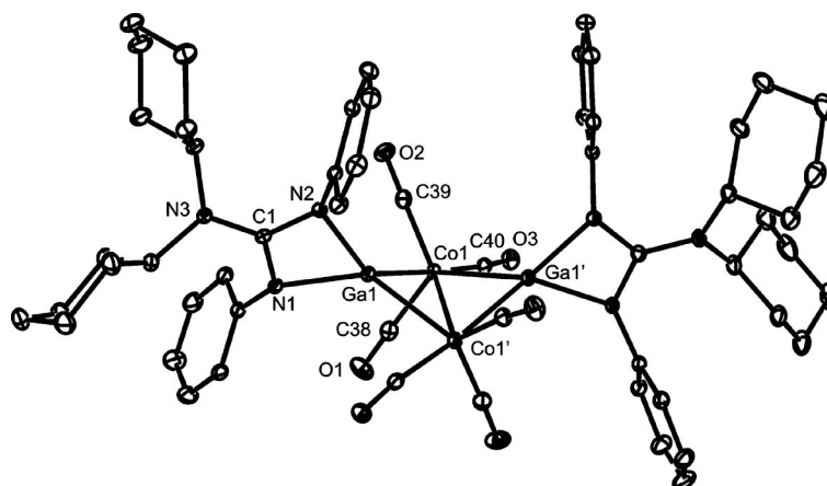
Figure 2. Molecular structure of 4 (ORTEP, thermal ellipsoids shown at 25% probability level). Isopropyl groups and hydrogen atoms omitted for clarity. Selected bond lengths [Å] and angles [°]: Ga(1)–N(2) 1.9883(19), Ga(1)–N(1) 2.0236(19), Ga(1)–Co(1) 2.3801(8), Ga(1)–Co(1') 2.3865(6), Co(1)–Co(1') 2.7725(9), N(1)–C(1) 1.361(3), C(1)–N(2) 1.365(3), C(1)–N(3) 1.371(3); N(2)–Ga(1)–N(1) 66.78(8), Co(1)–Ga(1)–Co(1') 71.13(3), Ga(1)–Co(1)–Ga(1') 96.77(3), N(1)–C(1)–N(2) 108.15(19), N(1)–C(1)–N(3) 126.1(2), N(2)–C(1)–N(3) 125.7(2). Symmetry transformation used to generate equivalent atoms: ' : -x, y, -z + 1/2 .
