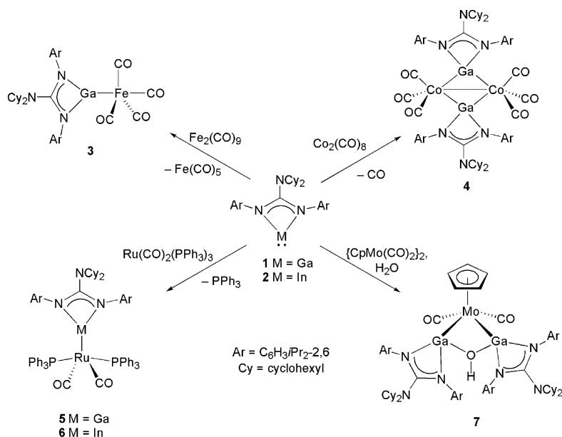
Scheme 1. Syntheses of compounds 3 – 7 .
